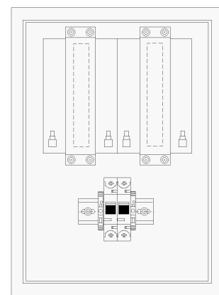
Internal View
